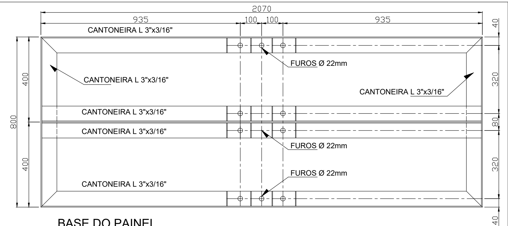
BASE DO PAINEL
